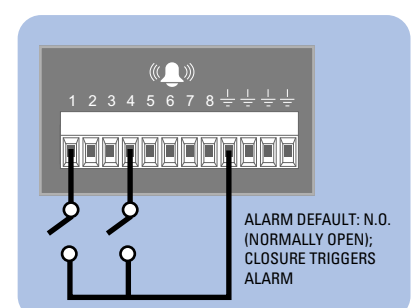
Figure 5. Alarm Connections
